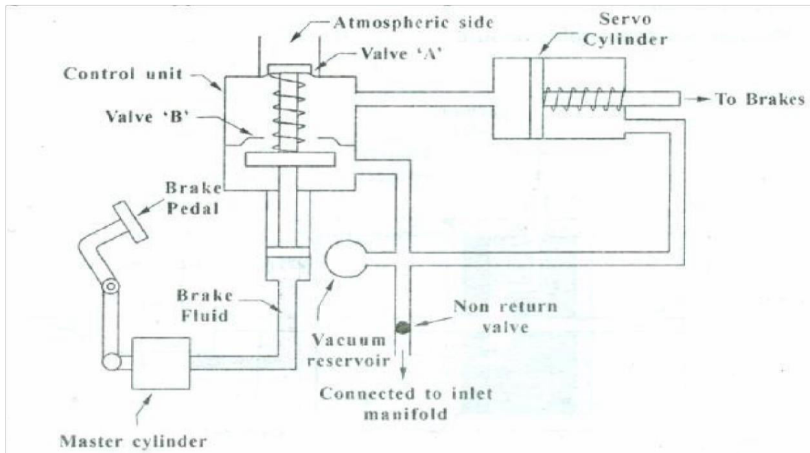
Fig: Vacuum Servo Brake
