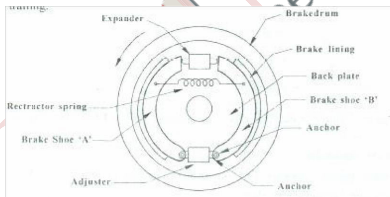
Fig: Components or a Drum Brake
