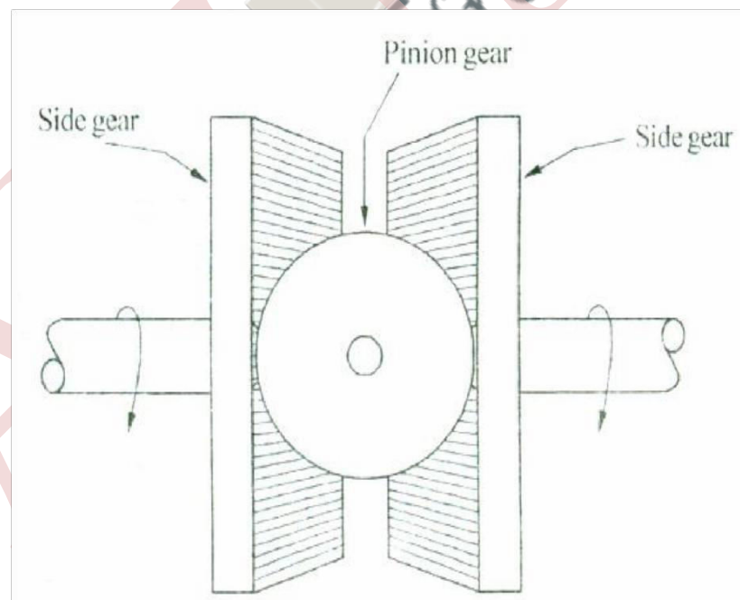
Fig (b): Differential
