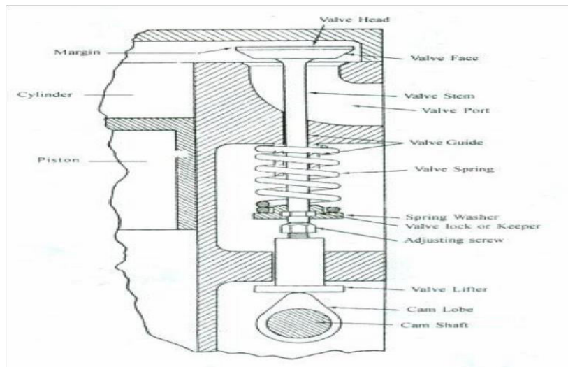
Fig: Detailed view of side valve mechanism
