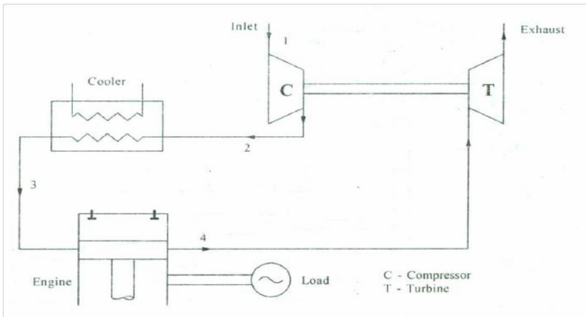
Fig: Super charging with turbine driven by engine exhaust
