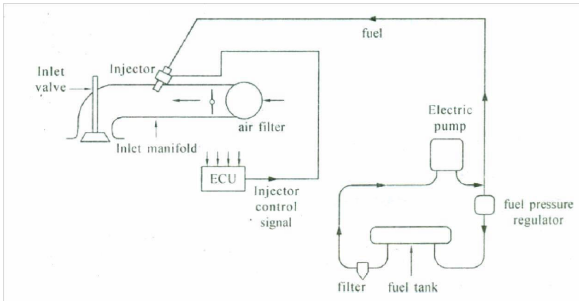
Fig: Electronic Fuel Injection System
