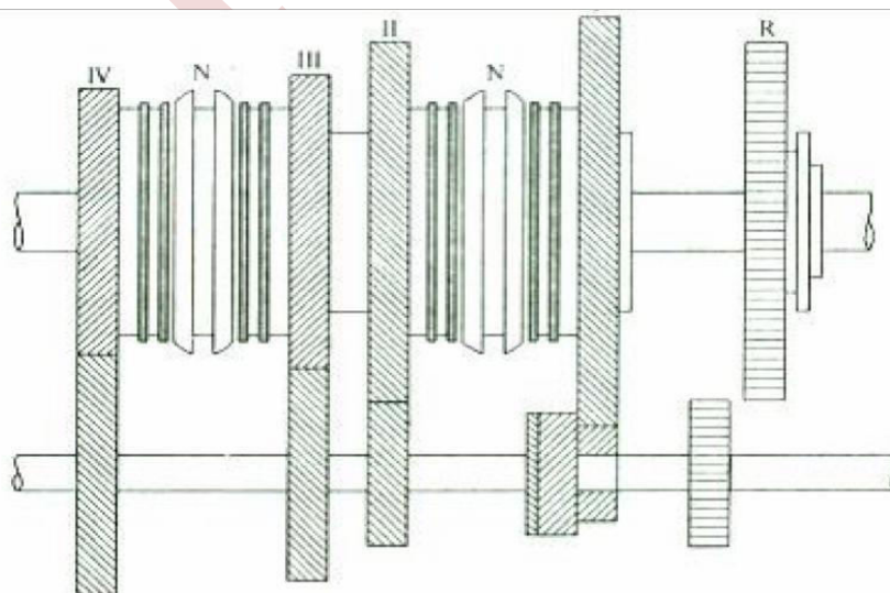
Fig. 5.11 : Four speed transmission with all forward speed synchronised
