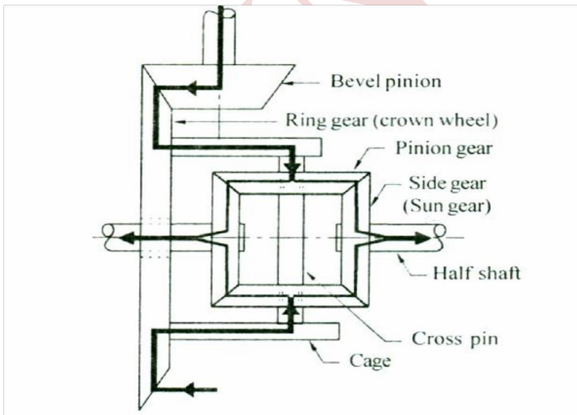
Fig (e): Power flow through nonslip differential on straight away .
