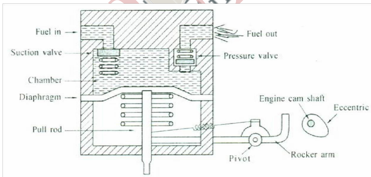
Fig: Mechanical Fuel pump
