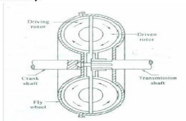
Fig: Fluid flywheel
