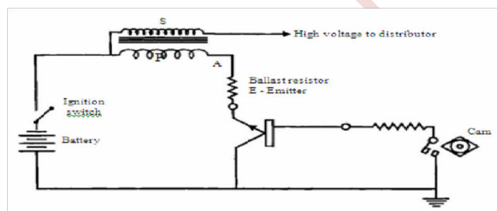
Figure: Transistorized Assisted Contact (TAC) Ignition System
