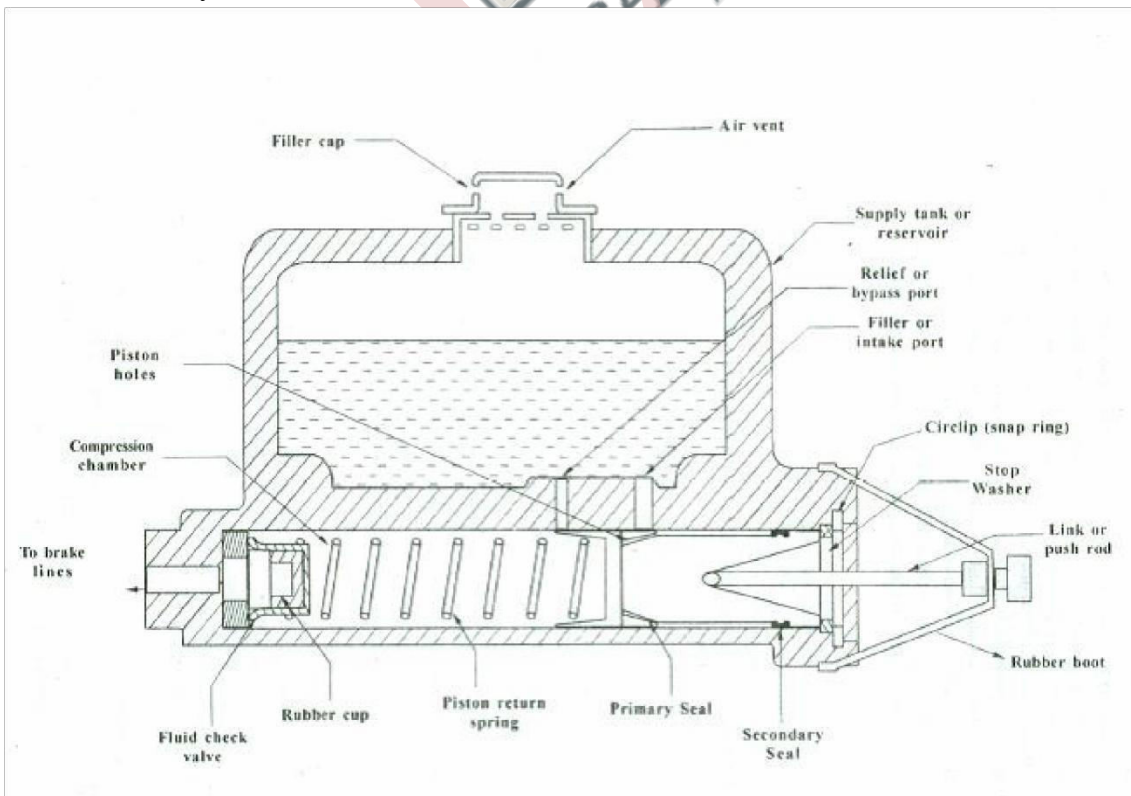
Fig: Master Cylinder
