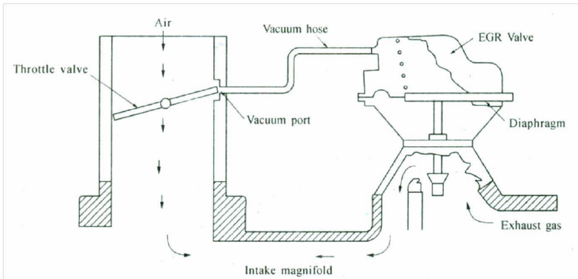
Fig: Schematic diagram of EGR system
