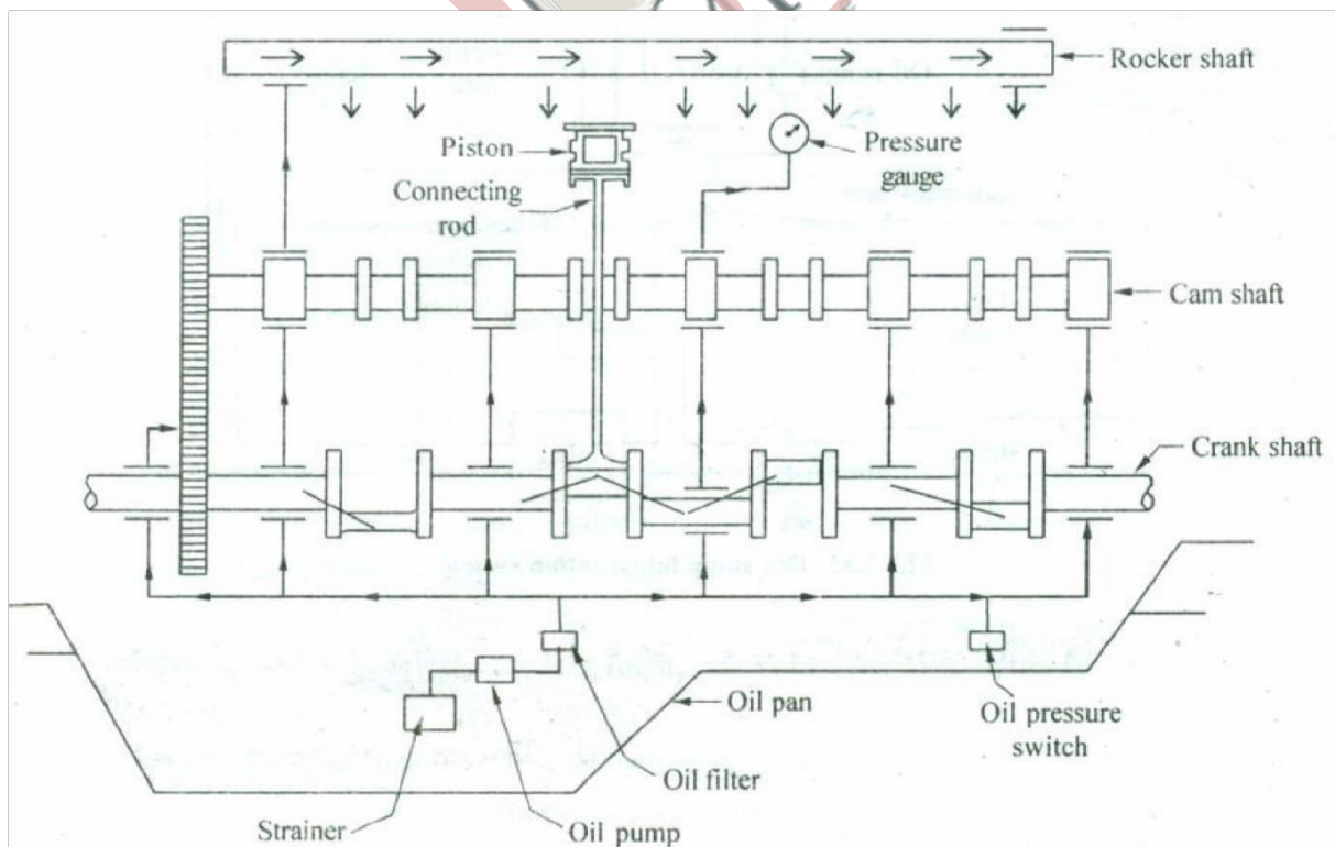
Fig: Full pressure feed lubrication system
