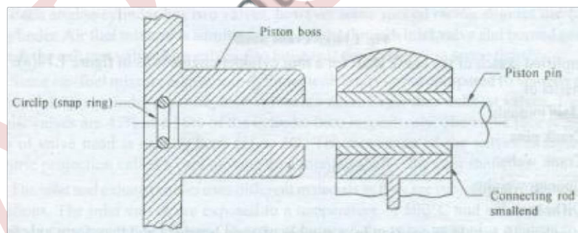
Fig: (b) Piston pin locked to connecting rod
