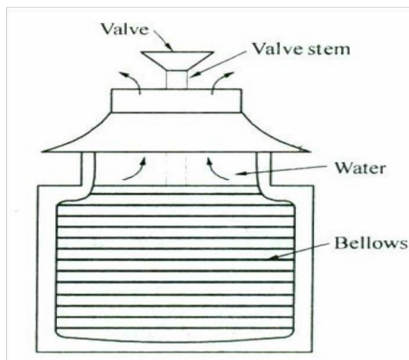
Fig. Bellows type thermostats
