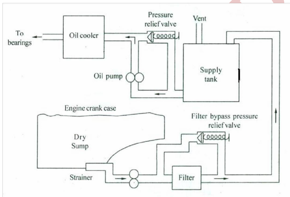
Fig. Dry sump lubrication system
