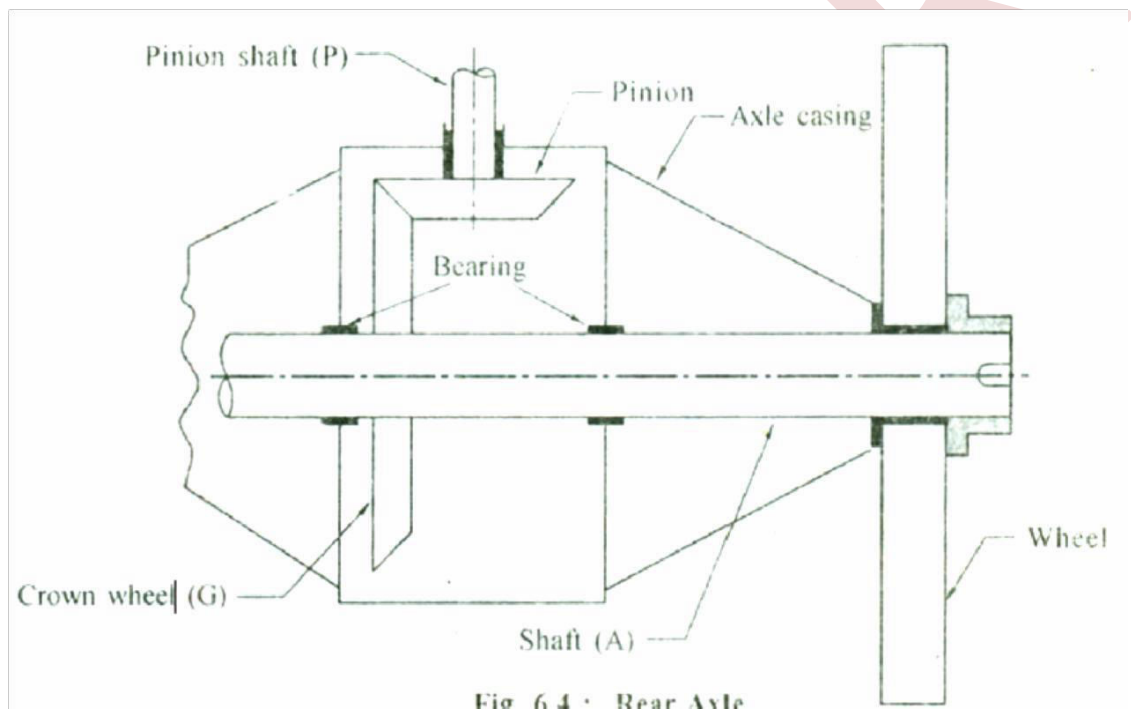
Fig: Rear Axle
