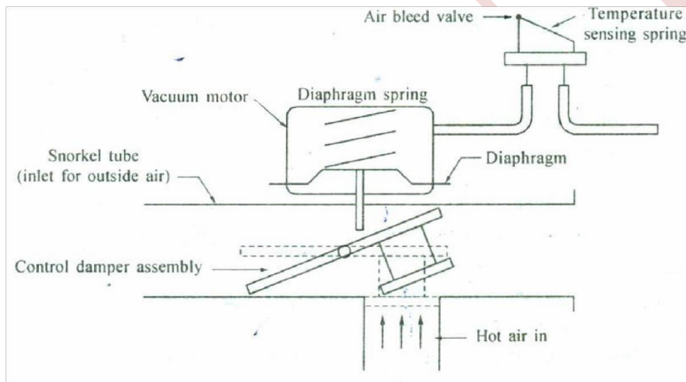
Fig: Thermostatic air cleaner
