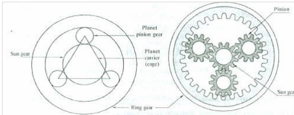
(a) Simplified view of planetary gear system (b) Planetary gear system
