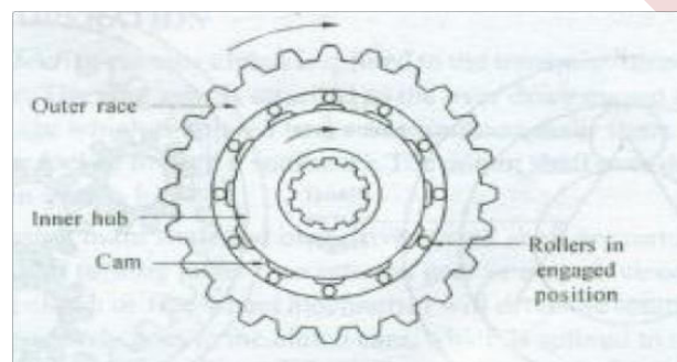
Fig: Over running clutch with rollers in engaged position (solid drive or coupling)
