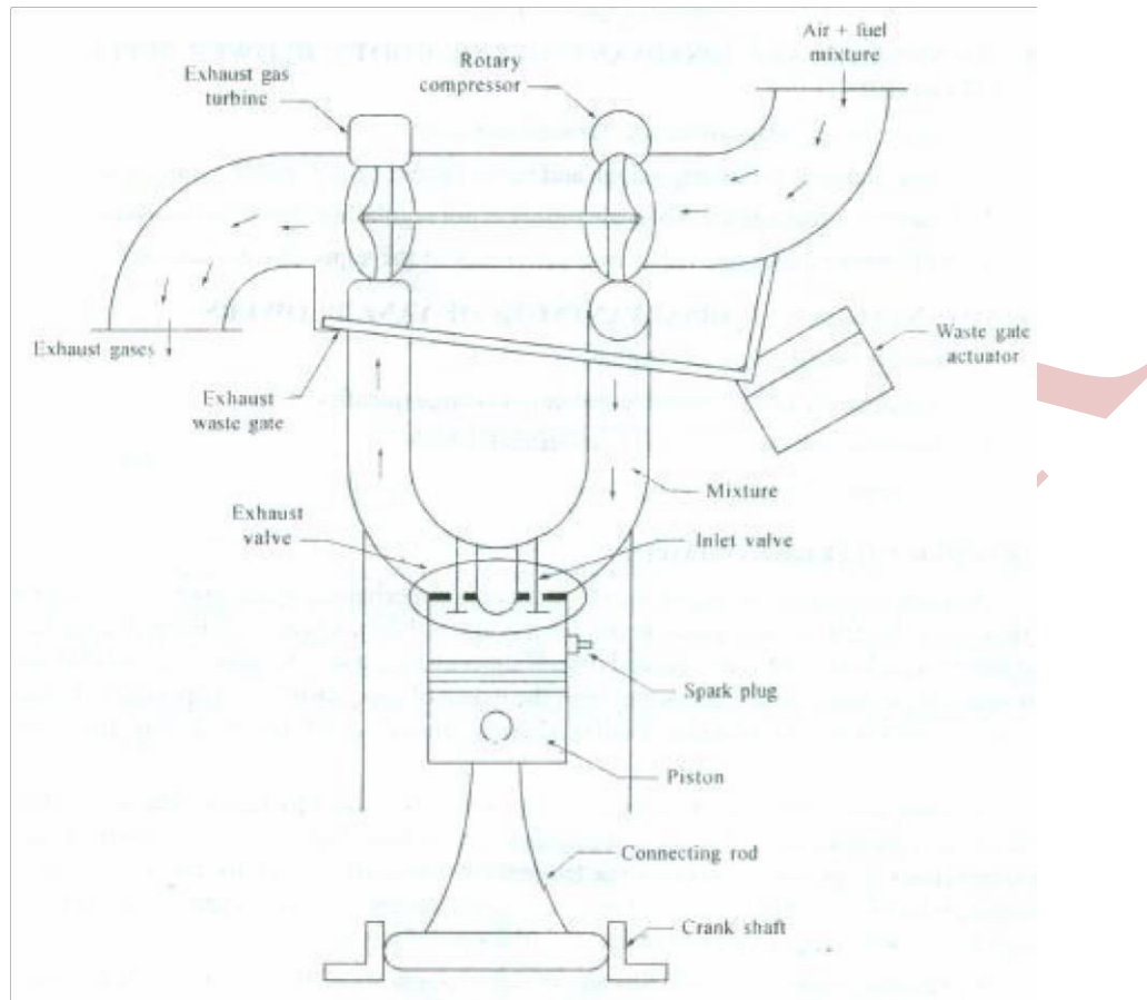
Fig: Exhaust turbo charging of a single cylinder engine
