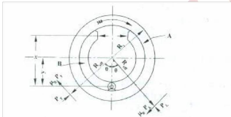
Fig: Forces in internally expanding shoe brake
