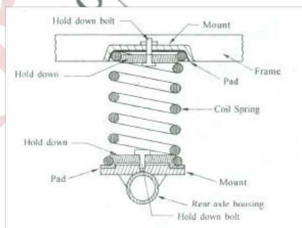
Fig: Coil Spring.
