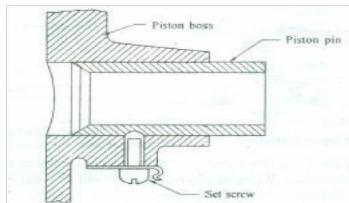
Fig: (a) Piston pin fastened to piston
