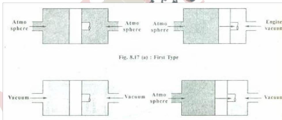
Fig: Second type; suspended vacuum type Brakes in released position & when brakes are applied.
