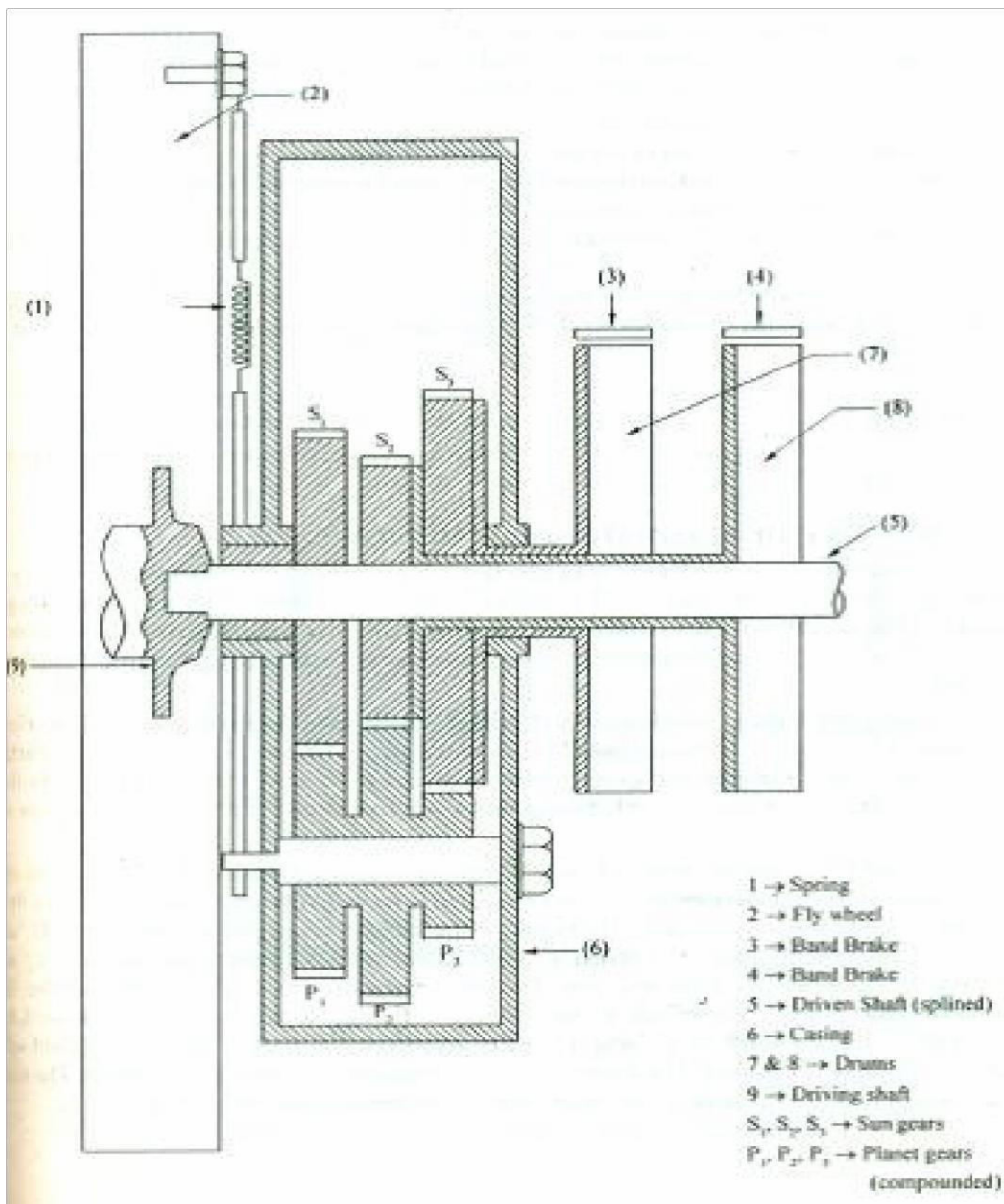
Fig: Epicyclic gearbox
