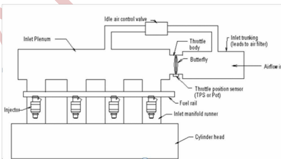
Fig : Multipoint injection
