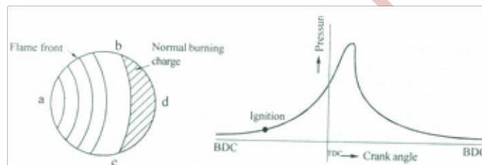
Fig: Normal combustion
