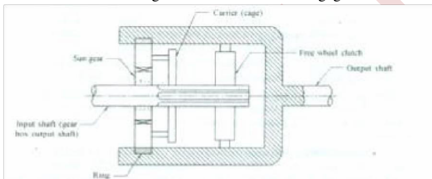
Fig: Overdrive
