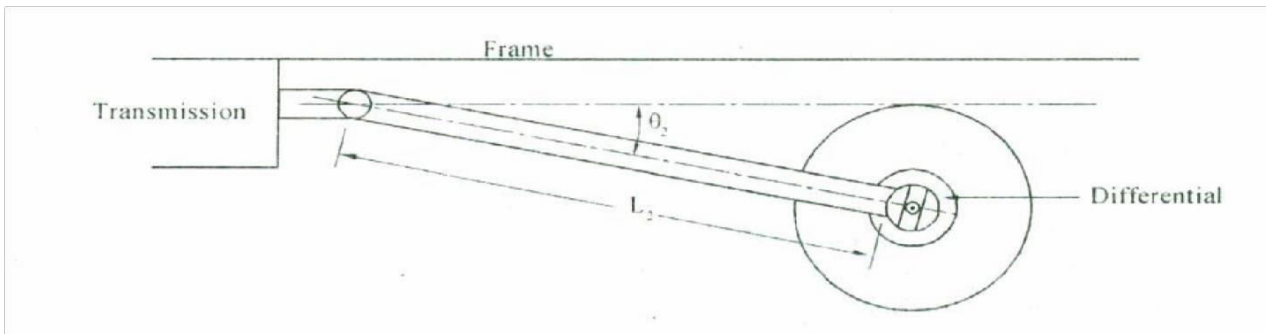
Fig: Propeller shaft length ( L_2 ) decreased
