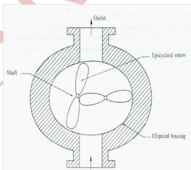
Fig: Root Supercharger
