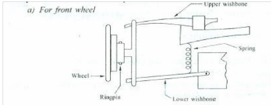
Fig: Independent front wheel suspension
