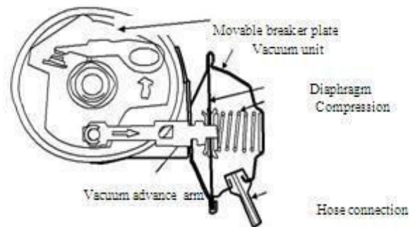
Figure 4.7: Vacuum Advance Mechanism
