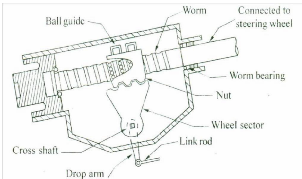
Fig: Recirculating ball type steering gear.
