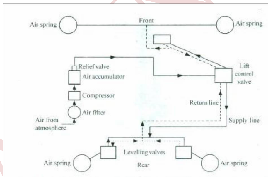
Fig: Layout of air suspension system
