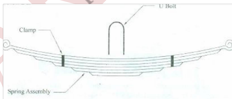
Fig: Semi elliptical leaf spring
