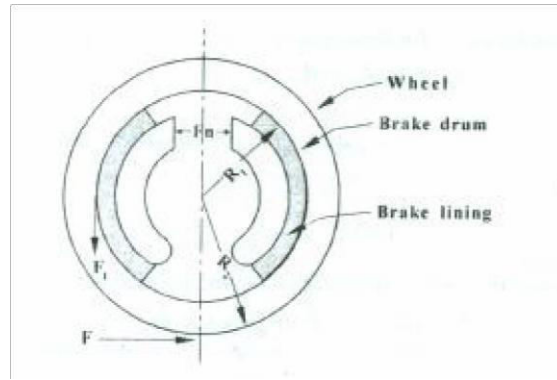
Fig: Braking effect
