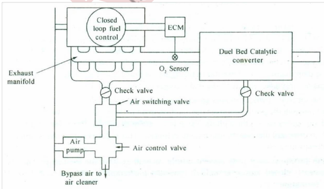
Fig: Air Injection System
