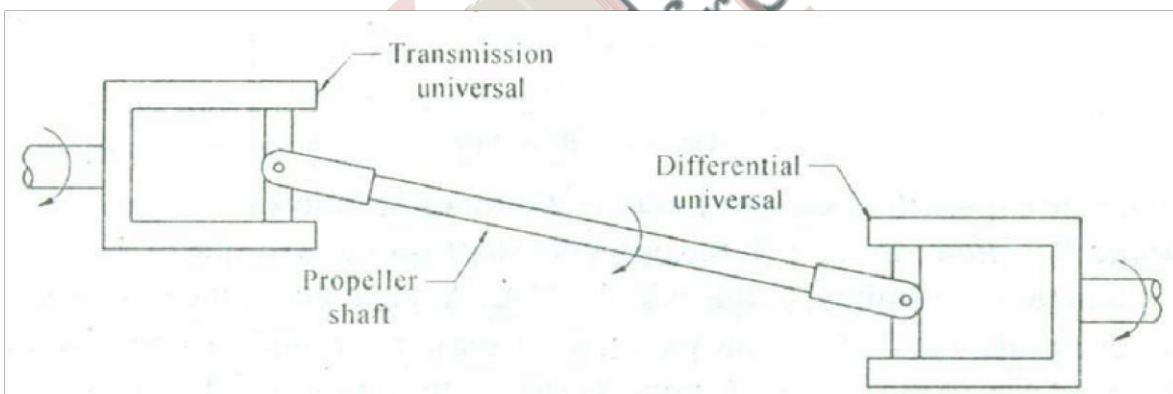
Fig: Universal joints in action. As rear axle moves up and down, universals allow drive angles to change without bending propeller shaft.
