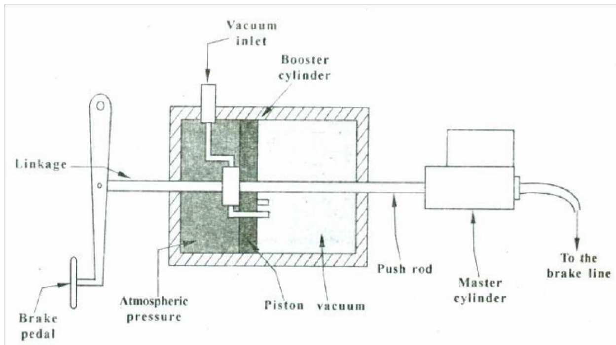
Fig: Simplified Power brake system
