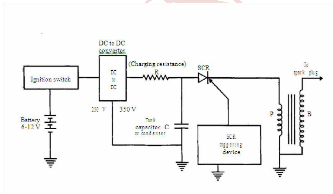
Figure: Capacitance Discharge Ignition System
