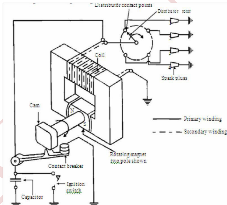
Figure 4.3: Schematic Diagram of Magneto Ignition System
