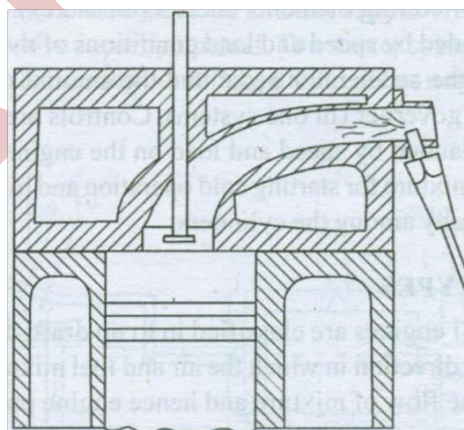
Fig: (a) Direct injection system
