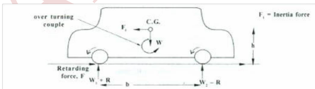
Fig (a): Weight transfer
