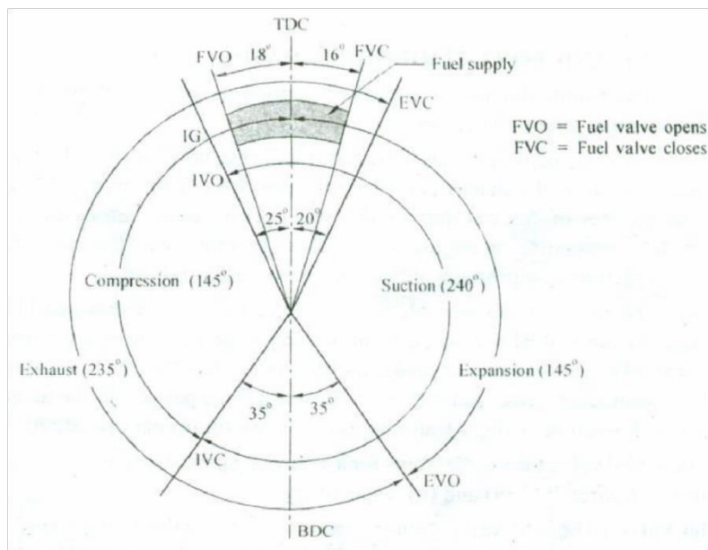
Fig: (b) Actual valve timing diagram for a 4S - Diesel engine
