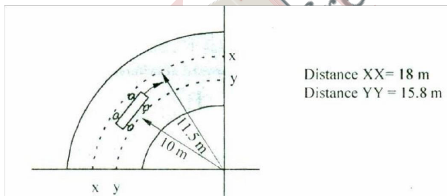
Fig (a): Distance travelled by inner and outer wheels when a car taking turn
