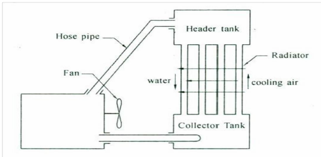
Fig (a): Thermosyphon Cooling System
