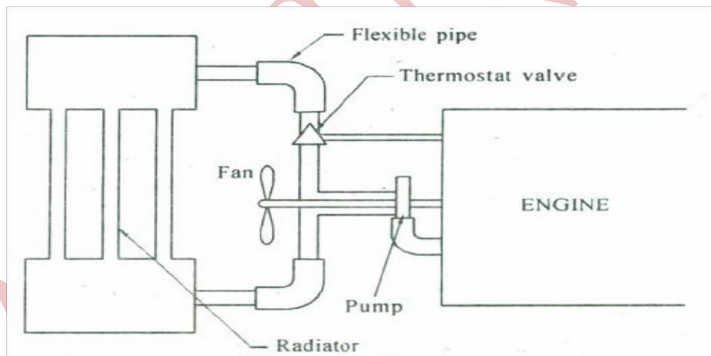
Fig (b): Pump Circulation System
