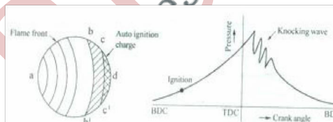
Fig: Combustion with Detonation
