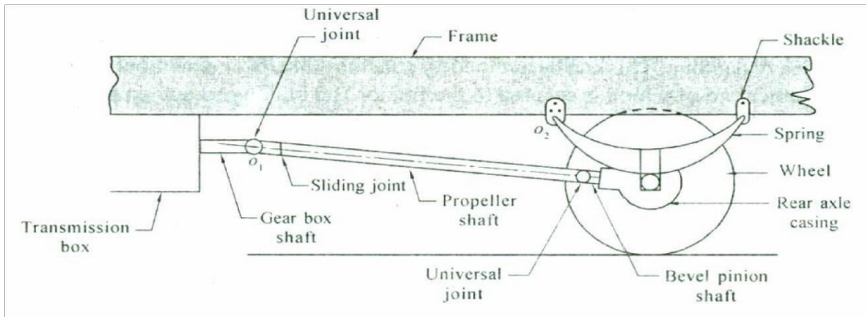
Fig: (a) Hotchkiss drive
