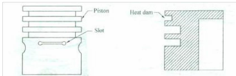
Fig: (a) Piston with horizontal slot Fig: (b) Heat dam construction
