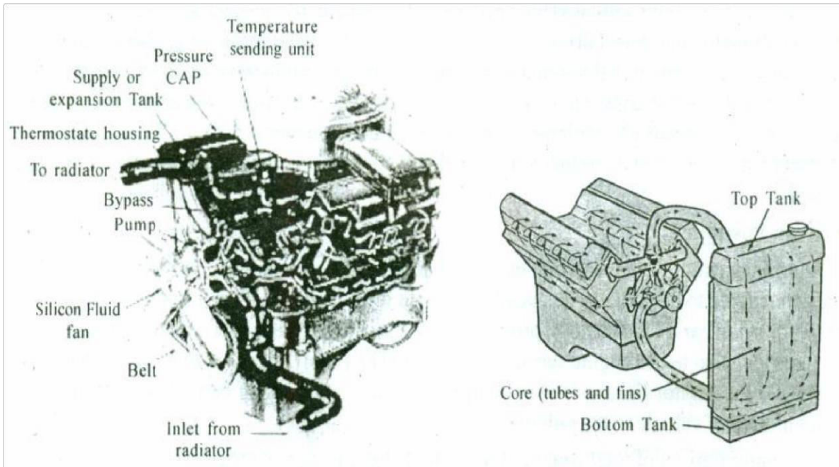
Fig (a): Coolant flows through an engine Fig (b) : Coolant flow path in a system using a down - flow radiator.
