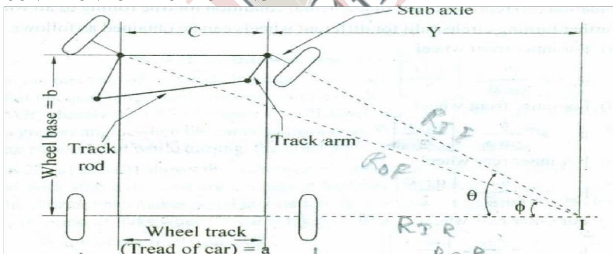
Fig: Condition for exact steering
