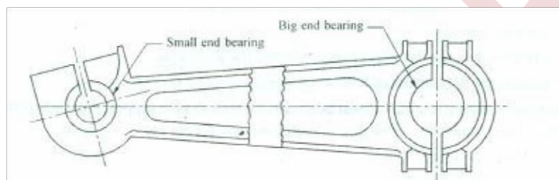
Fig: Connecting Rod
