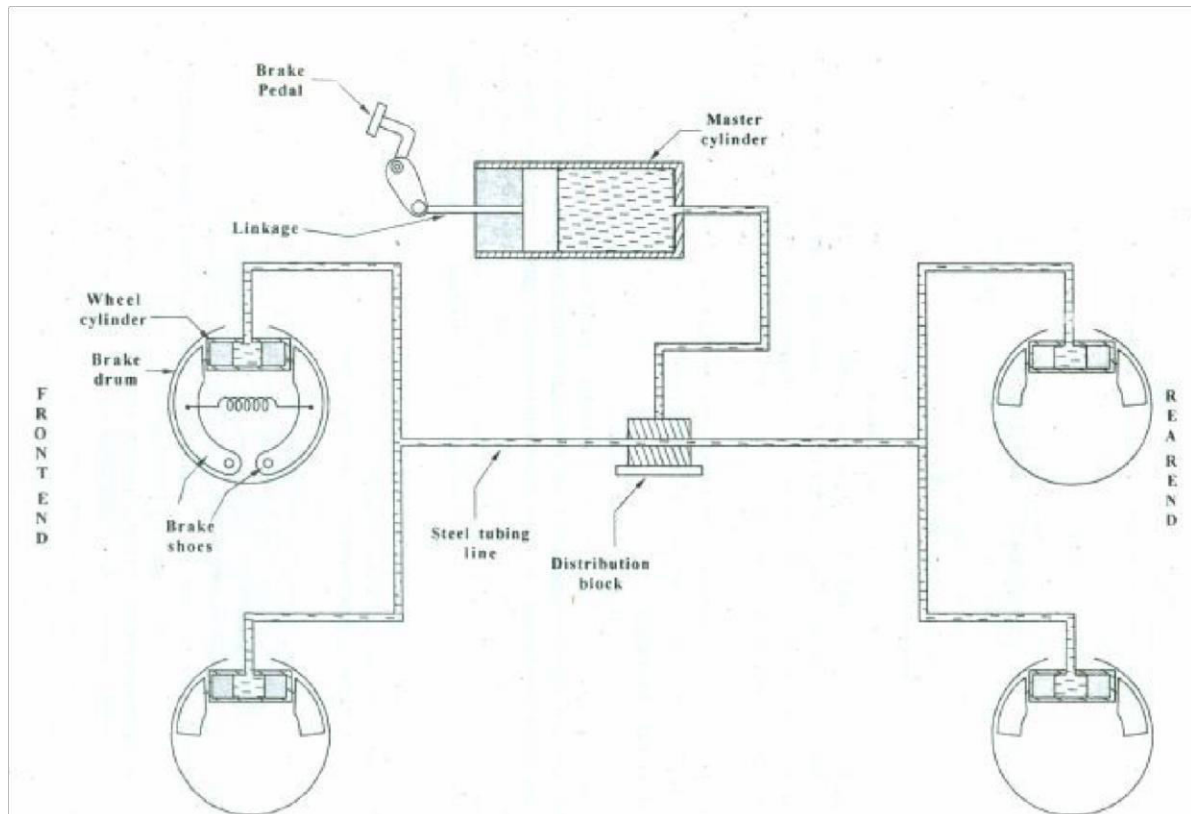
Fig: Hydraulic Brake system
