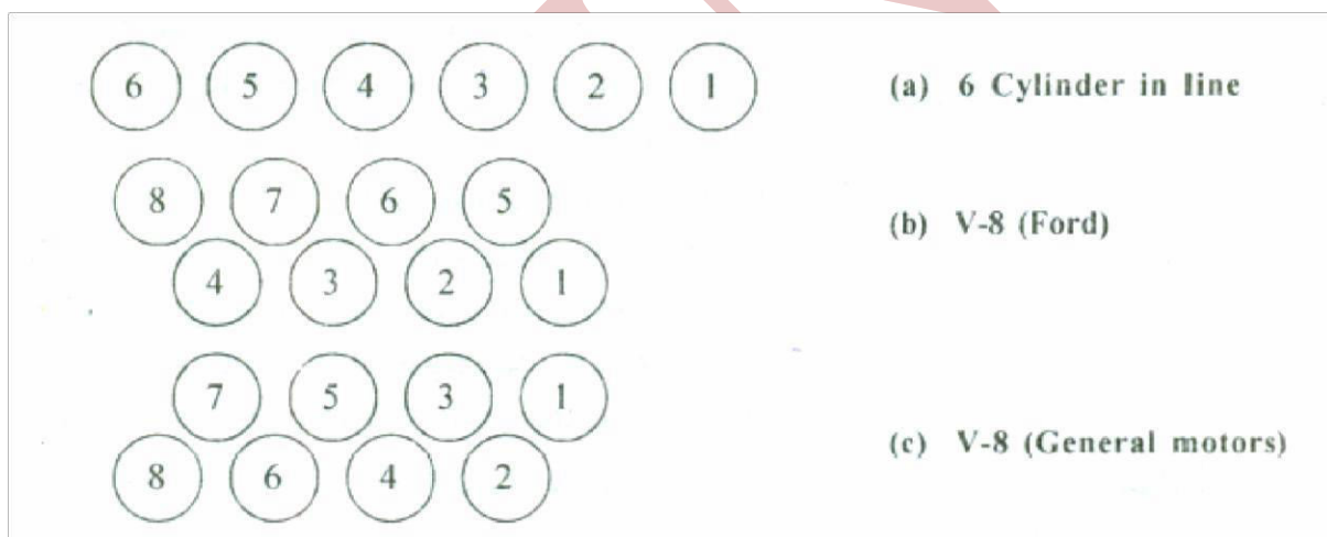
Fig numbering of engine cylinders
