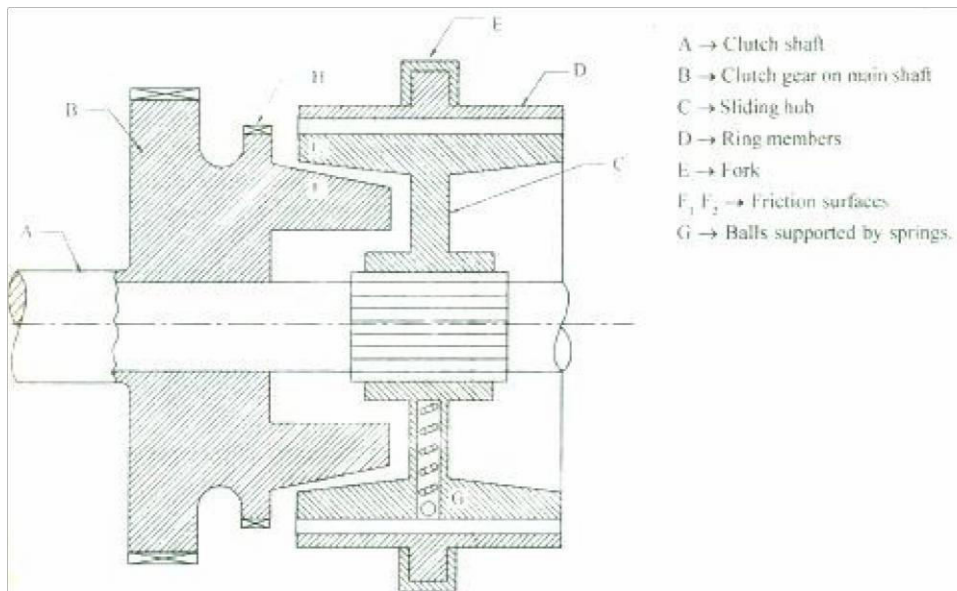
Fig. 5.9 Synchromesh device on higher gear side in a gear box.
