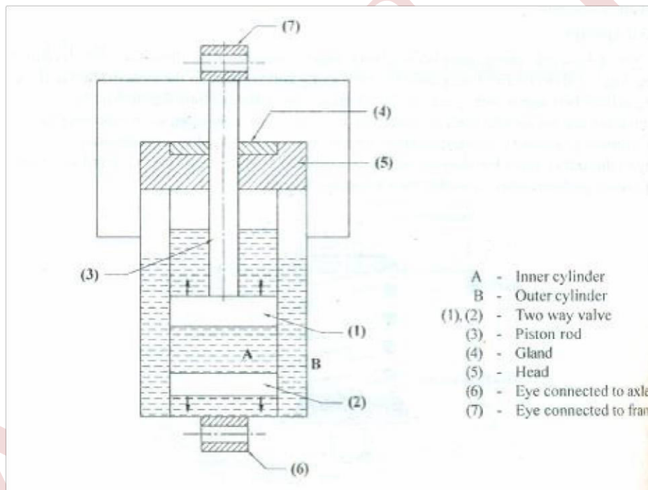
Fig: Illustrates the working of telescopic shock absorber
