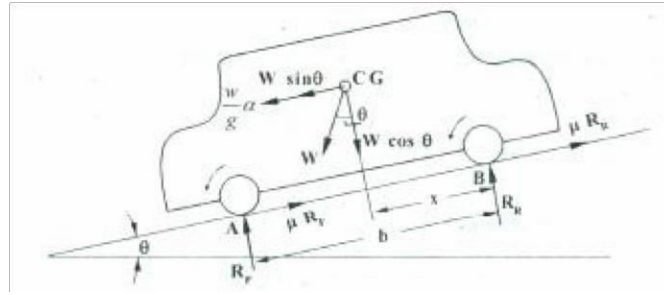
Fig (b): Forces on vehicle moving on an incline
