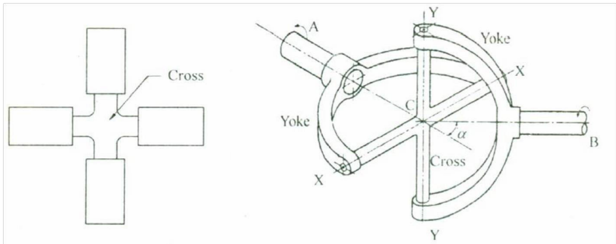
Fig: Hooke's joint. Shaft 'A' is transmitting torque in horizontal plane; shaft 'B' is transmitting the same at different angle.
