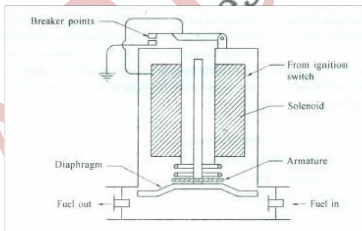
Fig: Electrical pump [S.U. type]
